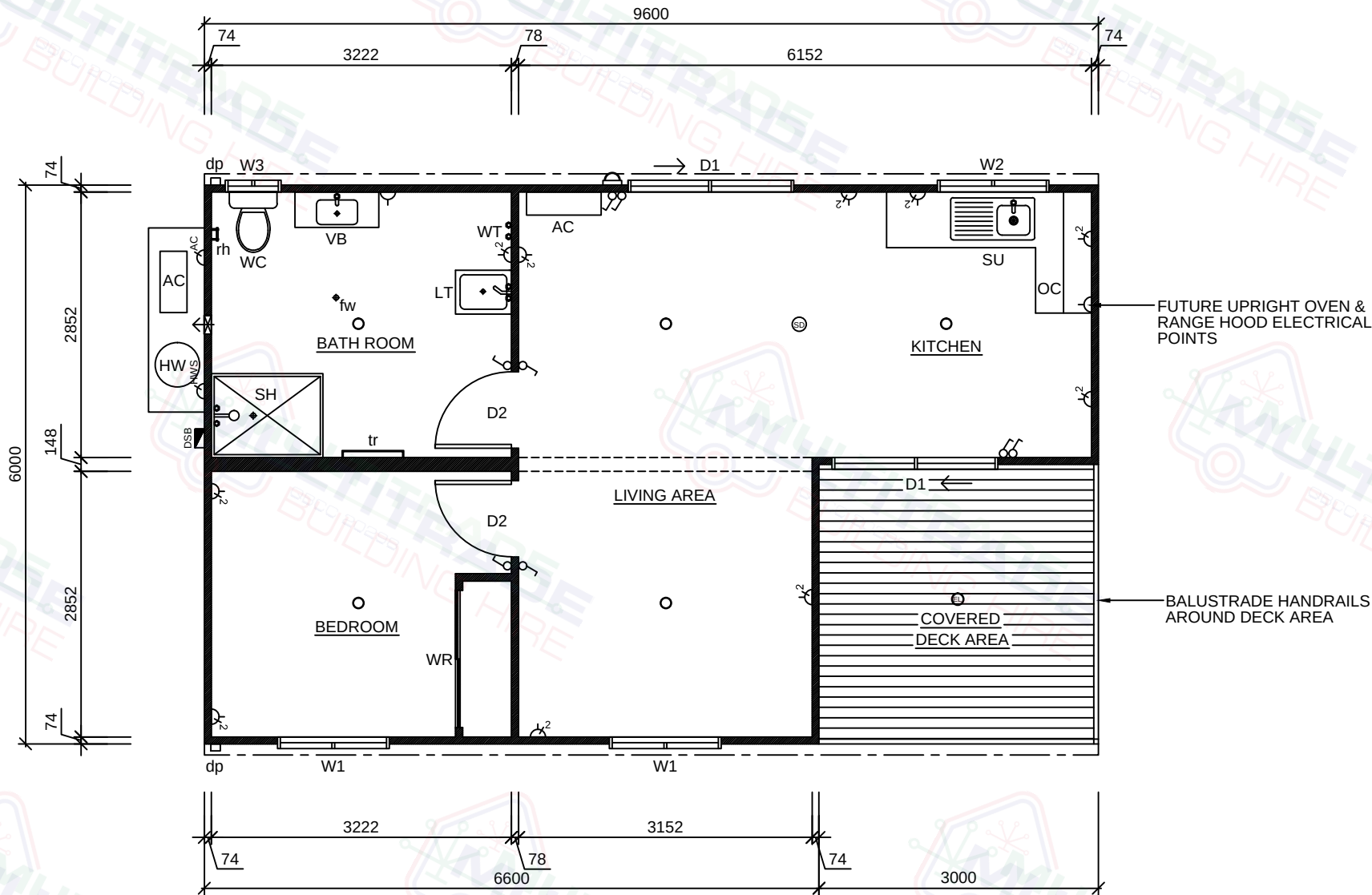
9.6x6.0m Single Bed Sitter Accommodation - Floor Plan
